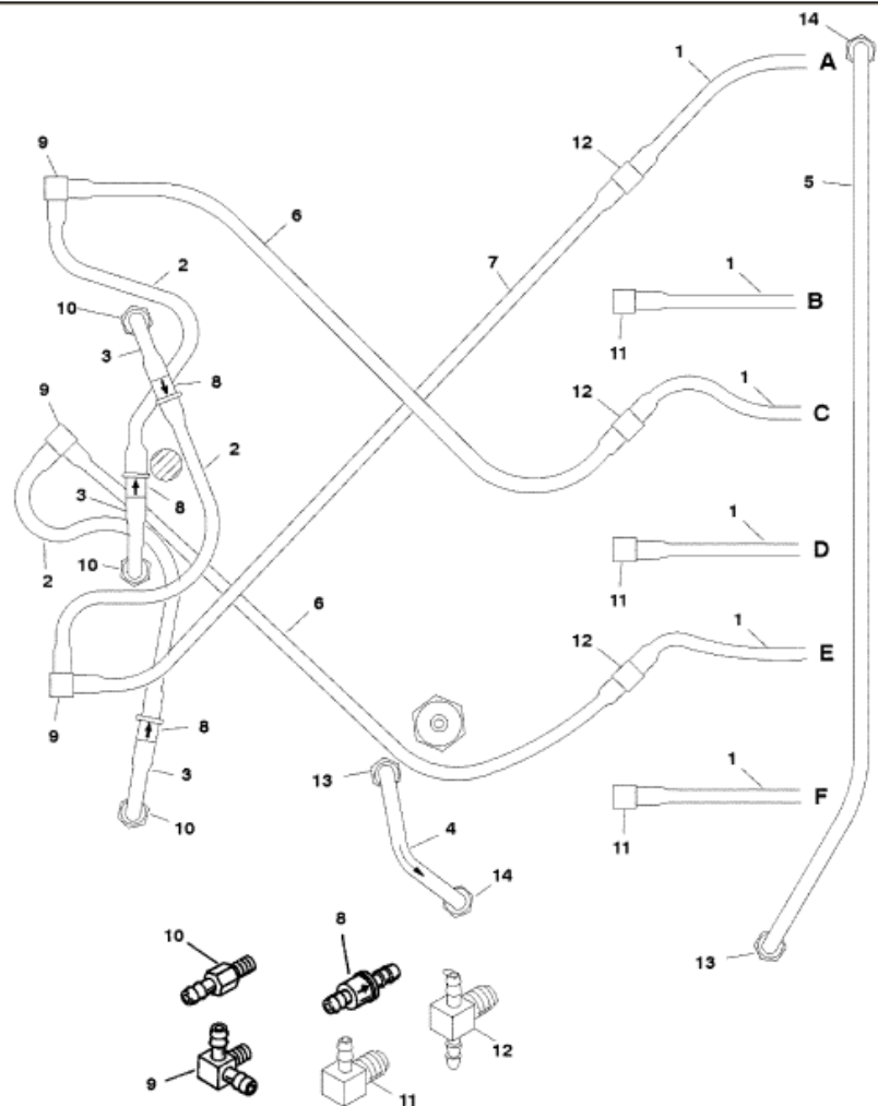
A THRU F - TUBING IS CONTINUED ON PORT SIDE
